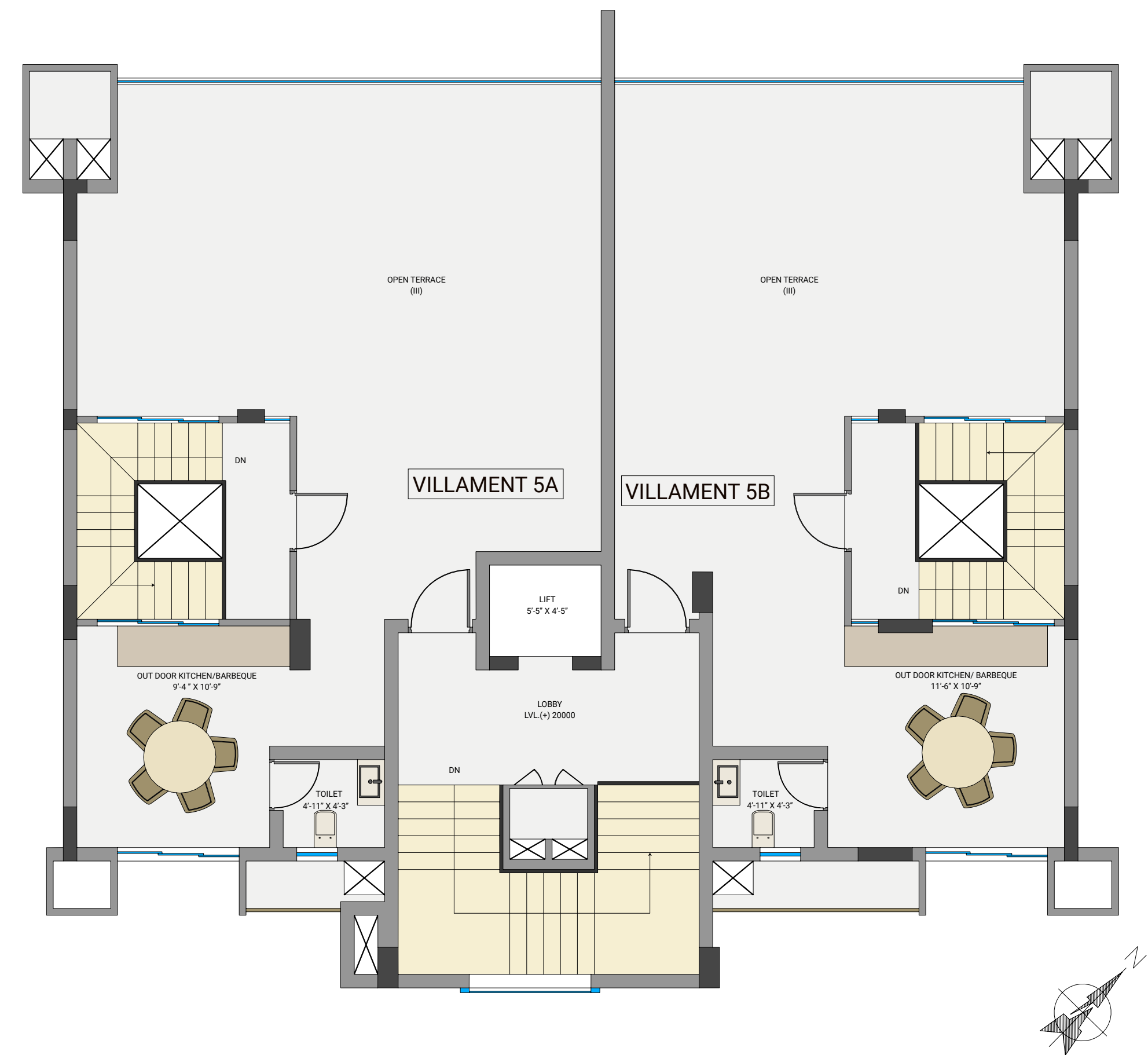
CENTER VILLAMENT 5A & VILLAMENT 5B - ROOF FLOOR PLAN
