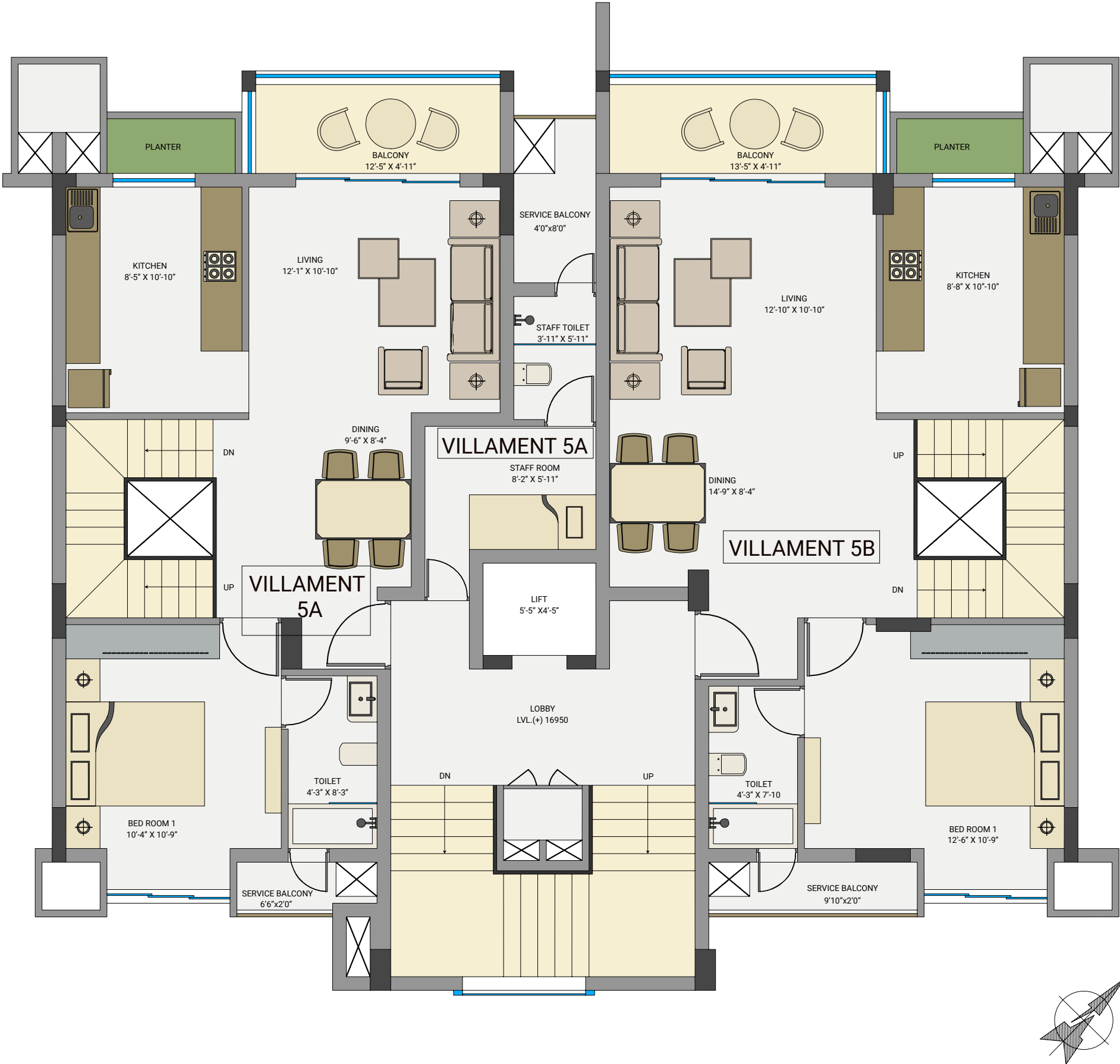
CENTER VILLAMENT 5A & VILLAMENT 5B - 5TH FLOOR PLAN (UPPER LEVEL PLAN)
