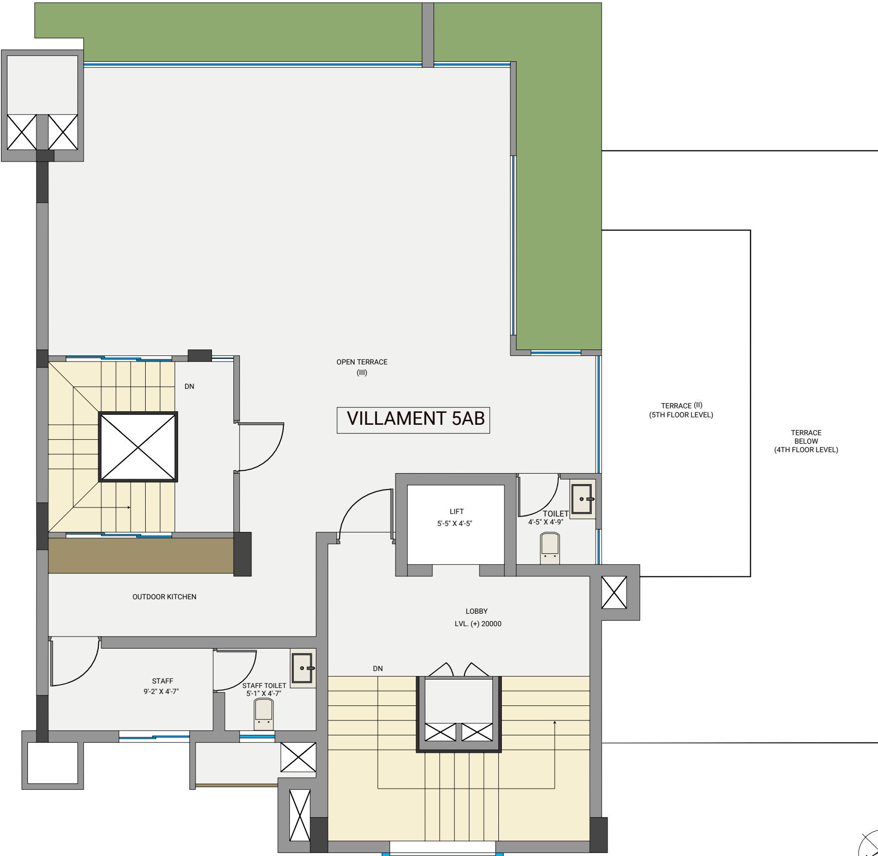
RIGHT SIDE CORNER VILLAMENT 5AB - ROOF FLOOR PLAN
