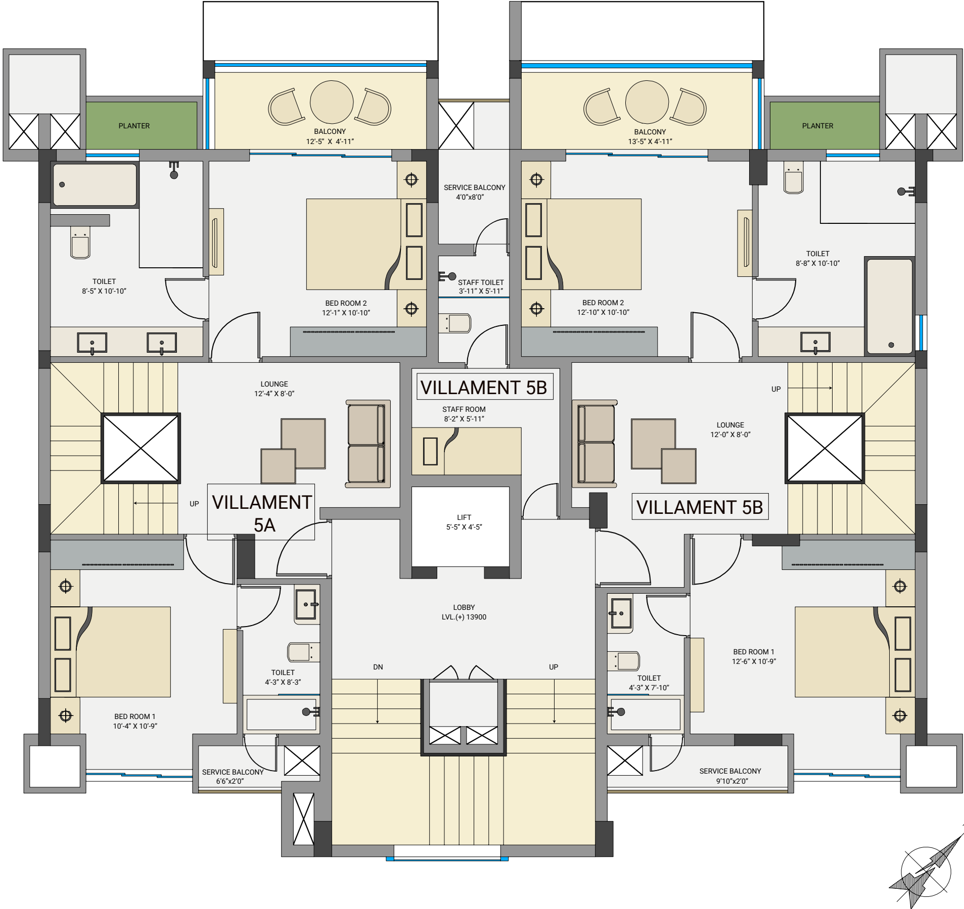
CENTER VILLAMENT 5A & VILLAMENT 5B - 4TH FLOOR PLAN (LOWER LEVEL PLAN)
